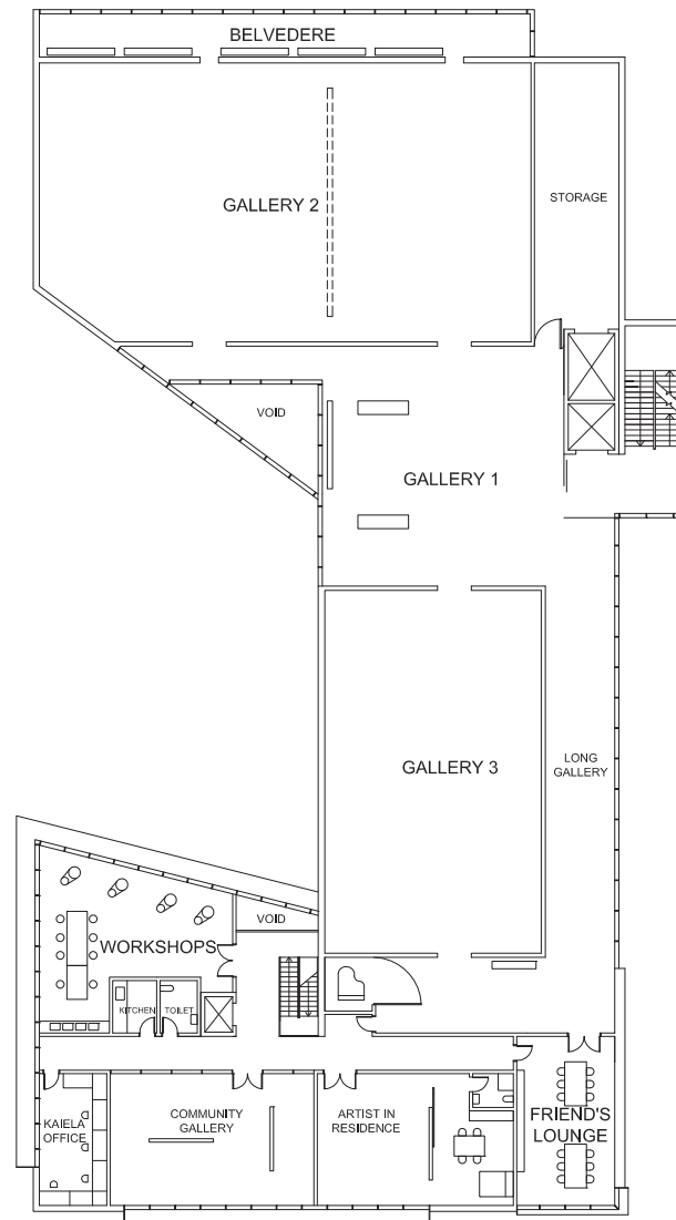
LEVEL 1 PLAN
