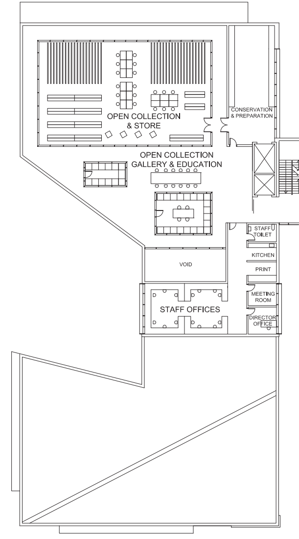
LEVEL 2 PLAN
