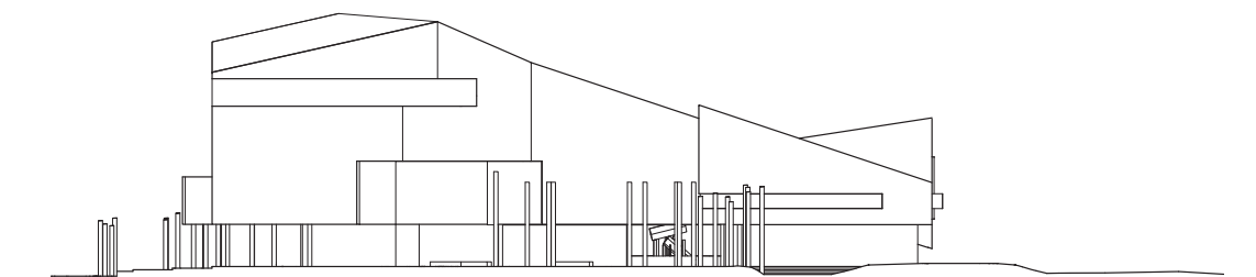
WEST ELEVATION
