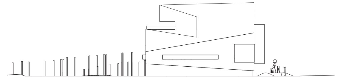
SOUTH ELEVATION
