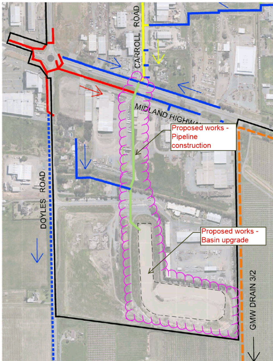
FIG01: Proposed Shepparton East Drainage Scheme Stage 1 A (shown as green line)
